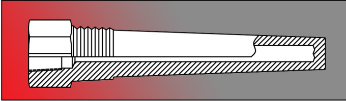
DRILLED THREADED THERMOWELLS, TAPERED SHANK See Document Number: TE-CO010109-TWPT-030
