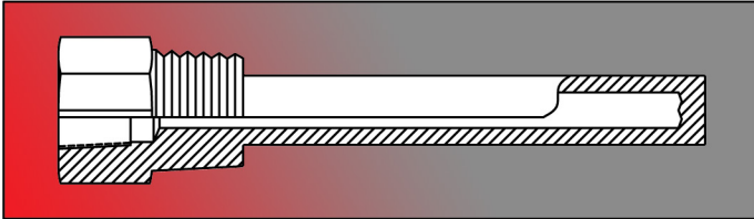
DRILLED THREADED THERMOWELLS, STRAIGHT SHANK See Document Number: TE-CO010109-TWPT-040
