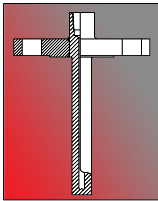
DRILLED FLANGED THERMOWELLS, TAPERED & STRAIGHT See Document Number: TE-CO010109-TWPT-080
