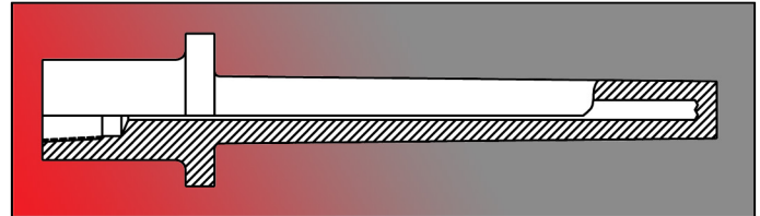
DRILLED VAN STONE THERMOWELLS, TAPERED SHANK See Document Number: TE-CO010109-TWPT-090
