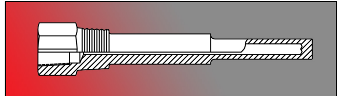
DRILLED THREADED THERMOWELLS, STEP DOWN SHANK See Document Number: TE-CO-010109-TWPT-060
