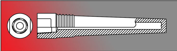
DRILLED THREADED THERMOWELLS, TAPERED SHANK, ALLOY METALS See Document Number: TE-CO010109-TWPT-050
