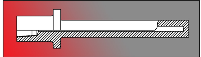
DRILLED VAN STONE THERMOWELLS, STRAIGHT SHANK See Document Number: TE-CO010109-TWPT-080
