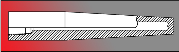
DRILLED WELD-IN THERMOWELLS See Document Number: TE-CO010109-TWPT-020
