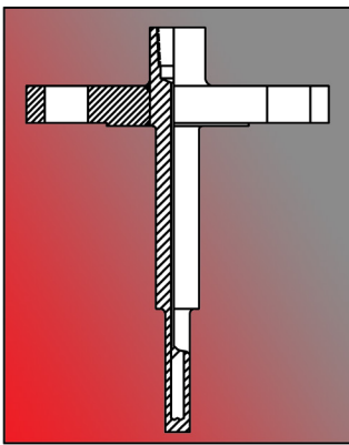
DRILLED FLANGED THERMOWELLS, STEP DOWN See Document Number: TE-CO010109-TWPT-060
