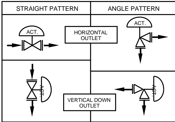
FIGURE 3: Installation Orientation
