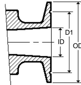
FIGURE 4 – Std. "Tri-Clamp®" End Connection
