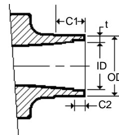
FIGURE 5 – Opt-24 Butt Weld End Connection
