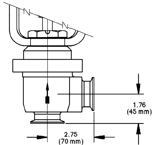
Model SCV-30 – Angle-Globe Body Sizes 3/4", 1" and 1-1/2"
