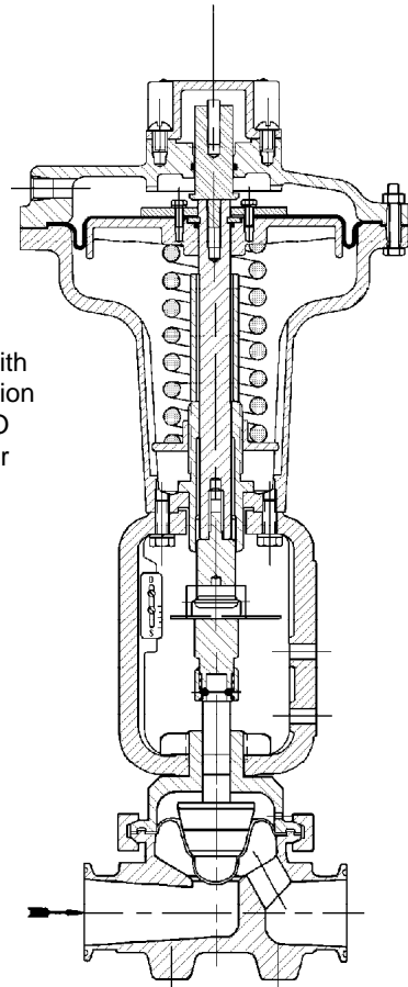
FIGURE 1 – STRAIGHT BODY
