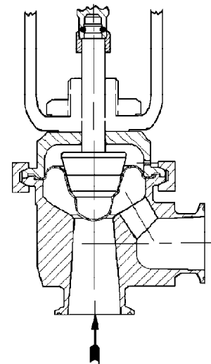
FIGURE 2 – ANGLE BODY
