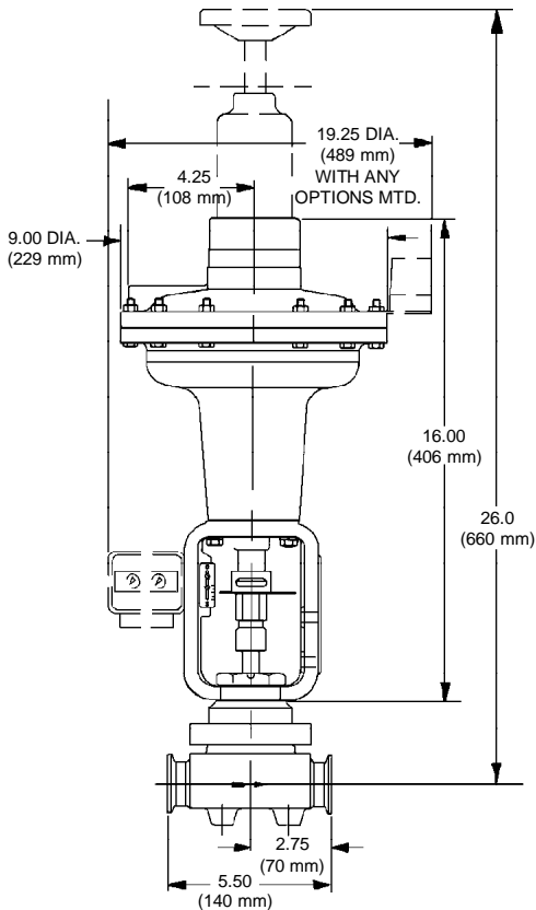
Model SCV-30 - Straight-Globe Body Sizes 3/4", 1" and 1-1/2"
