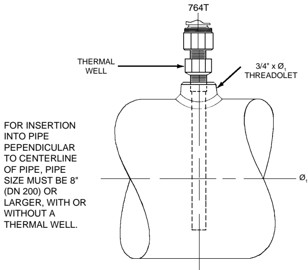
PIPE 8" (DN 200) Ø & LARGER
