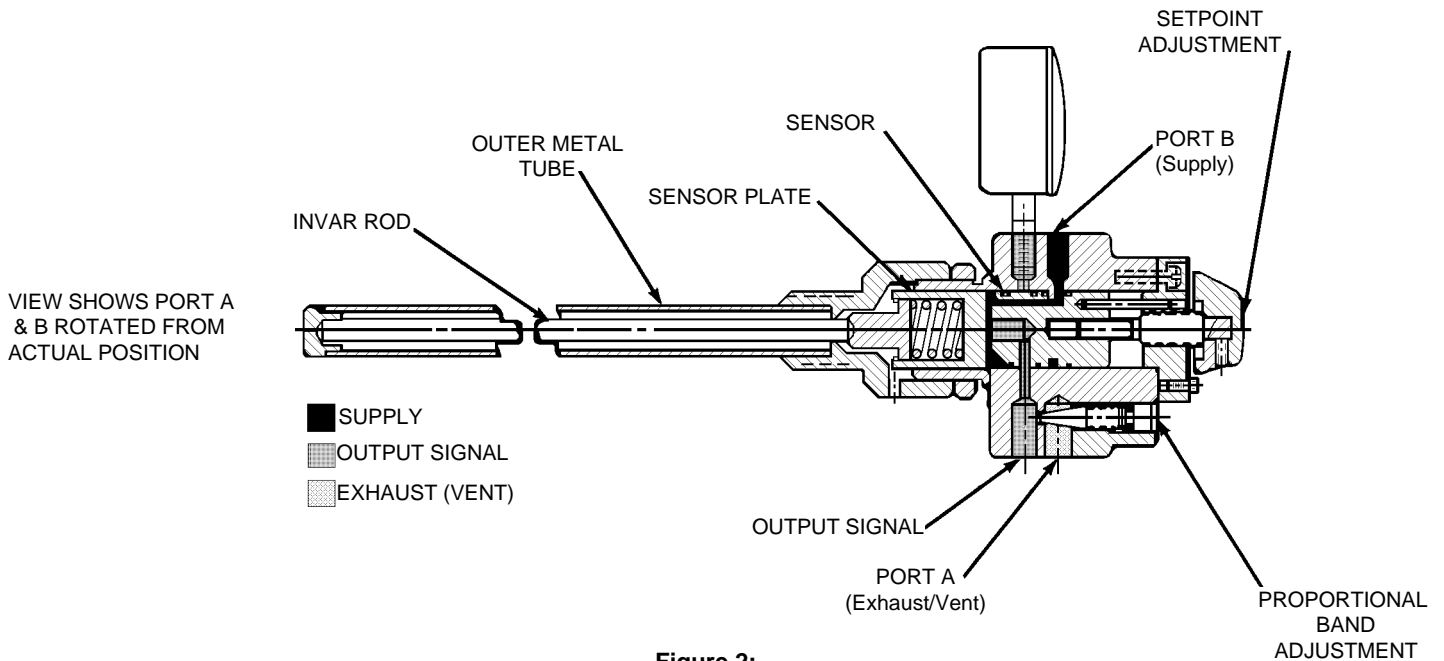
Figure 2: Direct Action 764T
