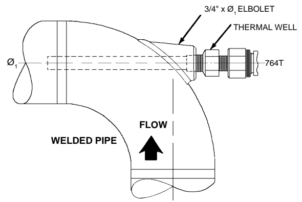
REQ'D: 2-1/2" (DN 65) THRU 6" (DN 150) OPTIONAL: 8" (DN 200) OR LARGER
