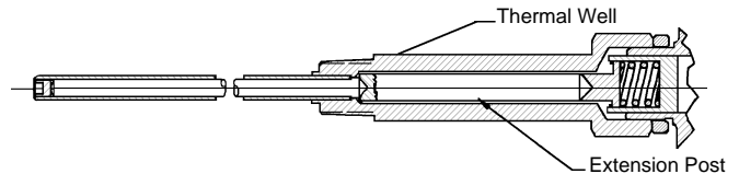
Figure 1: High Temperature Thermal Bulb (Opt. 63).
