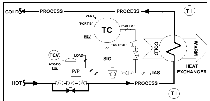
Figure 1: Typical Direct Cooling Application
