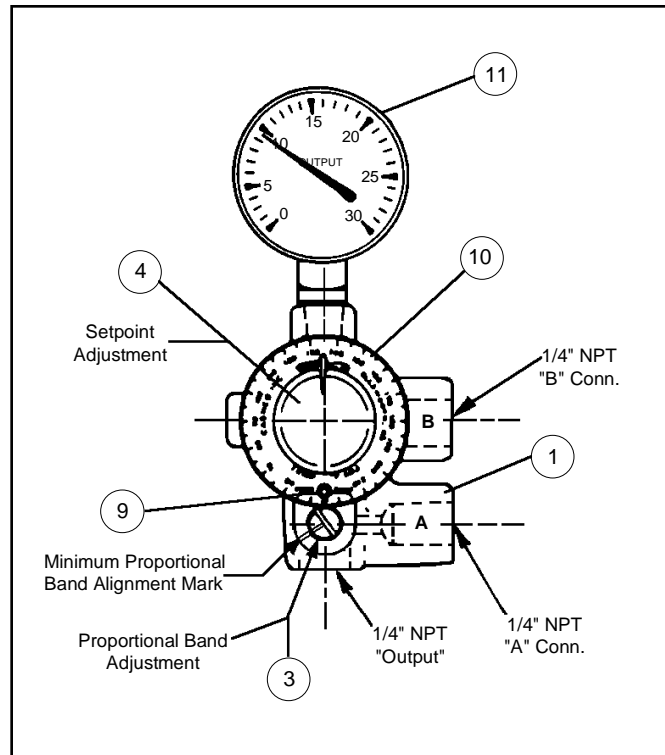
Figure 8: 764T End View
