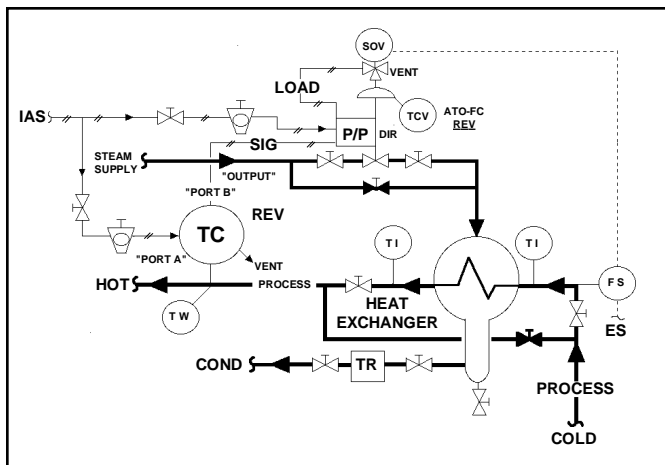
Figure 2: Typical Indirect Heating Application
